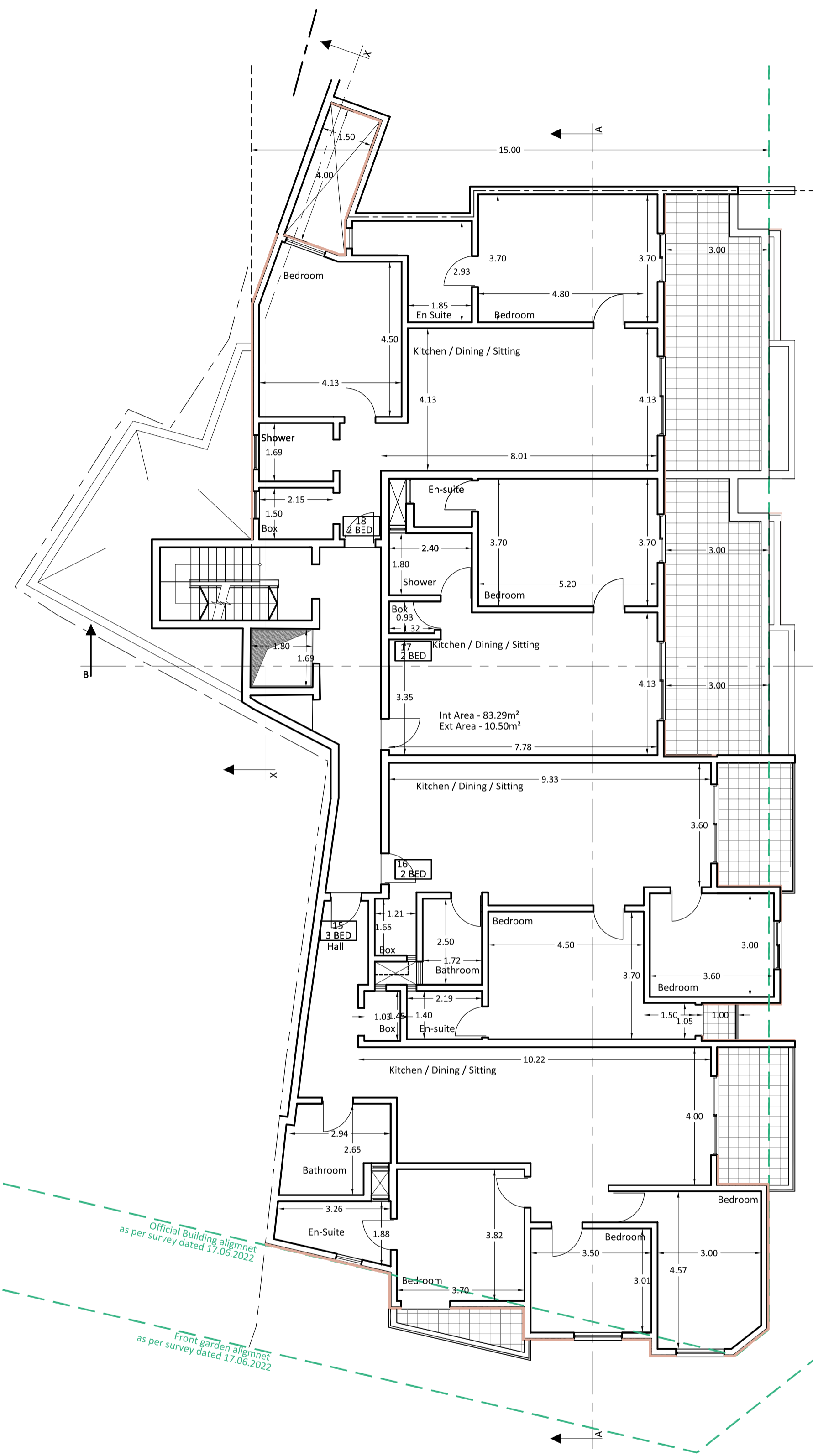
LEVEL 6 SCALE 1:100 PROPOSED
