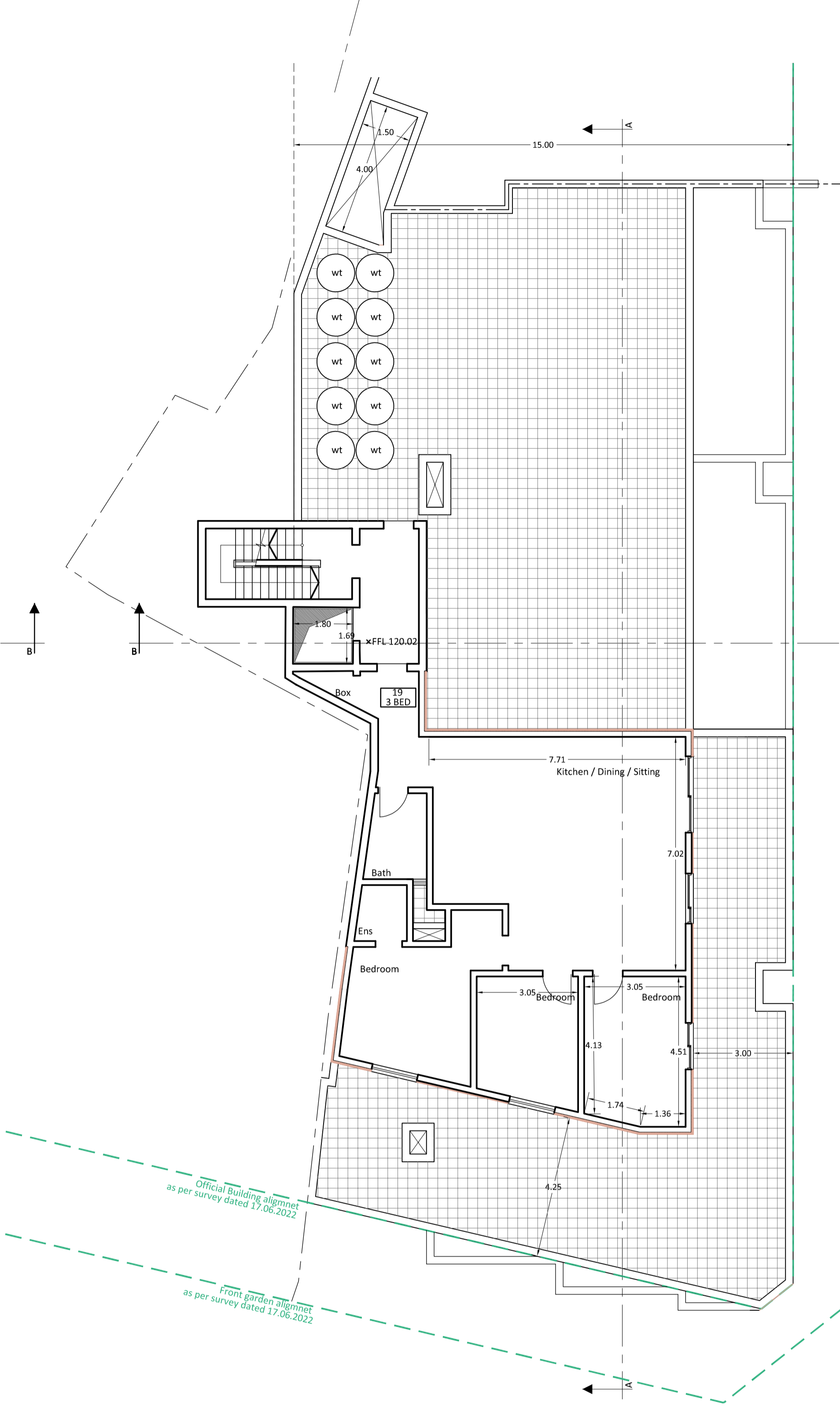
LEVEL 7 SCALE 1:100 PROPOSED
