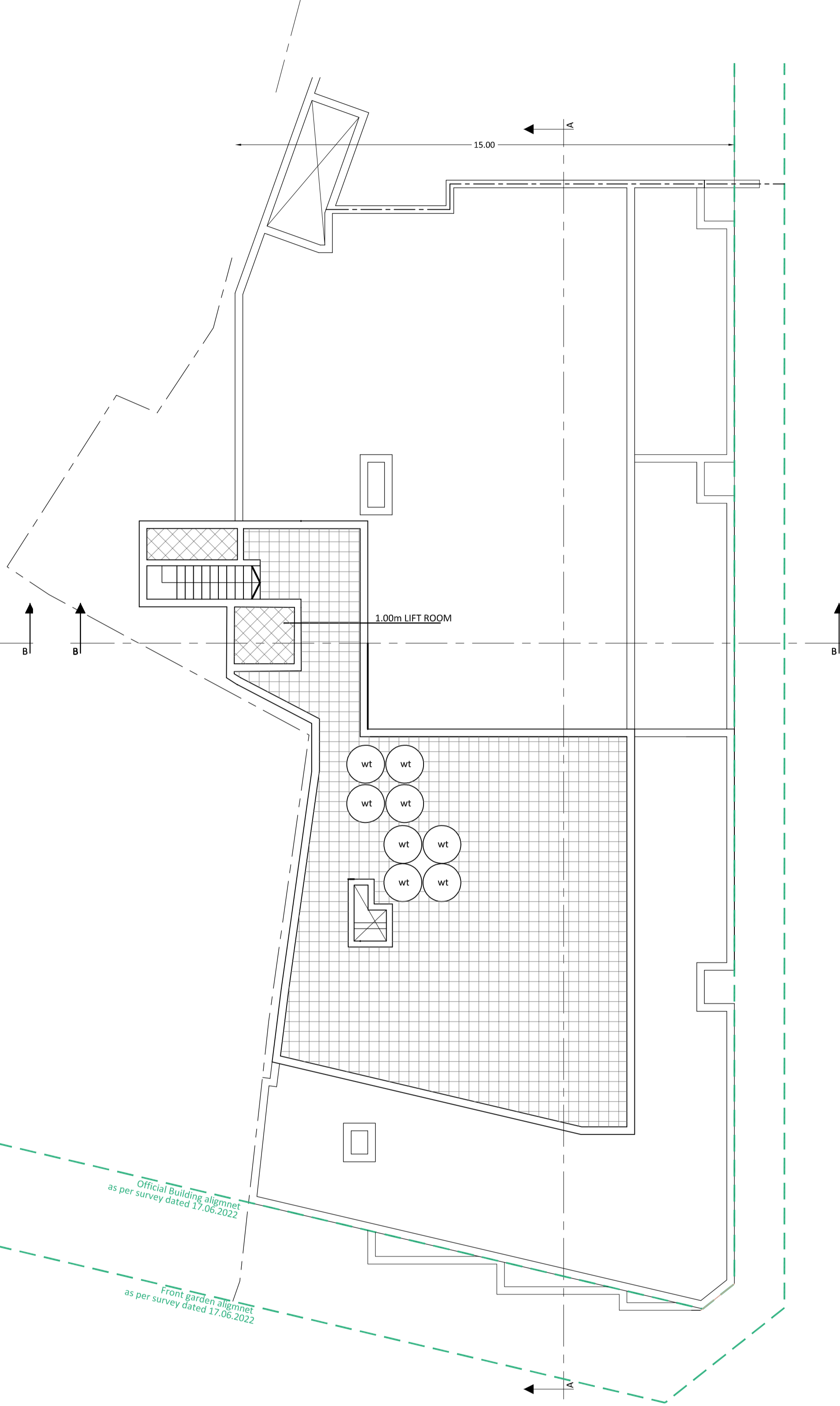
LEVEL 9 SCALE 1:100 PROPOSED
