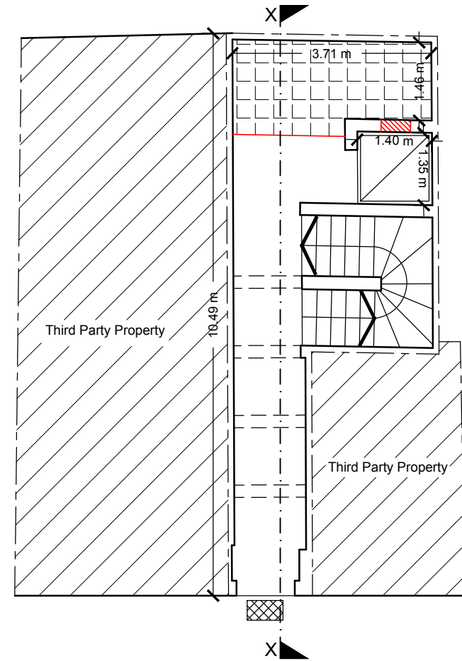
Proposed Ground Floor SCALE 1:100
