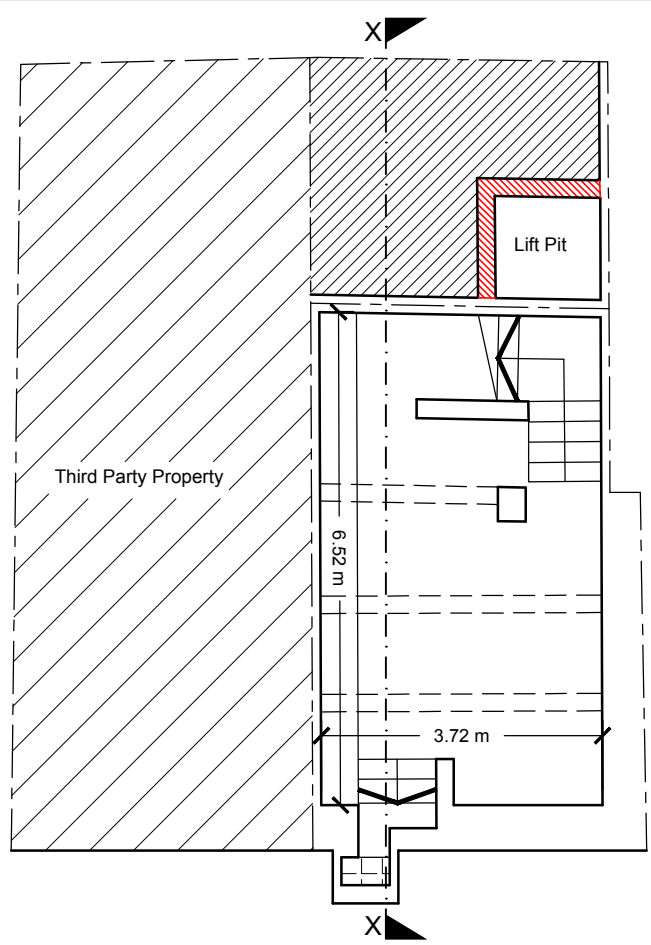
Proposed Basement SCALE 1:100
