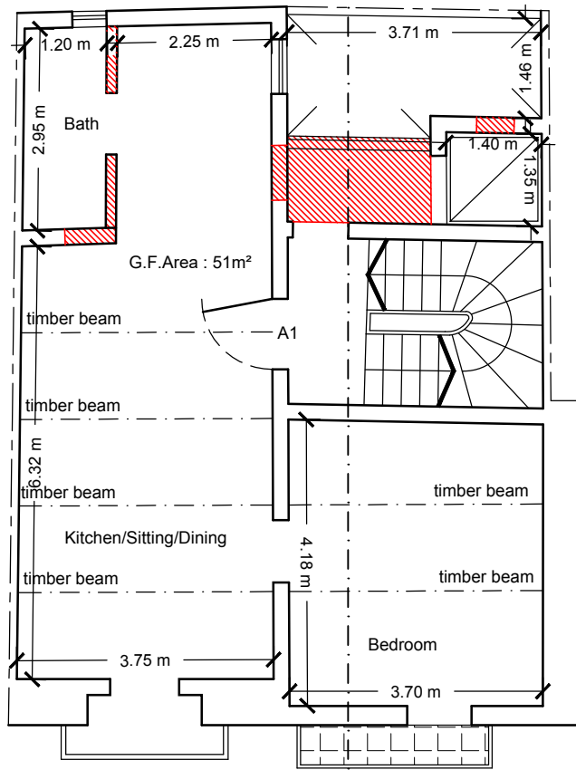
Proposed Second Floor
