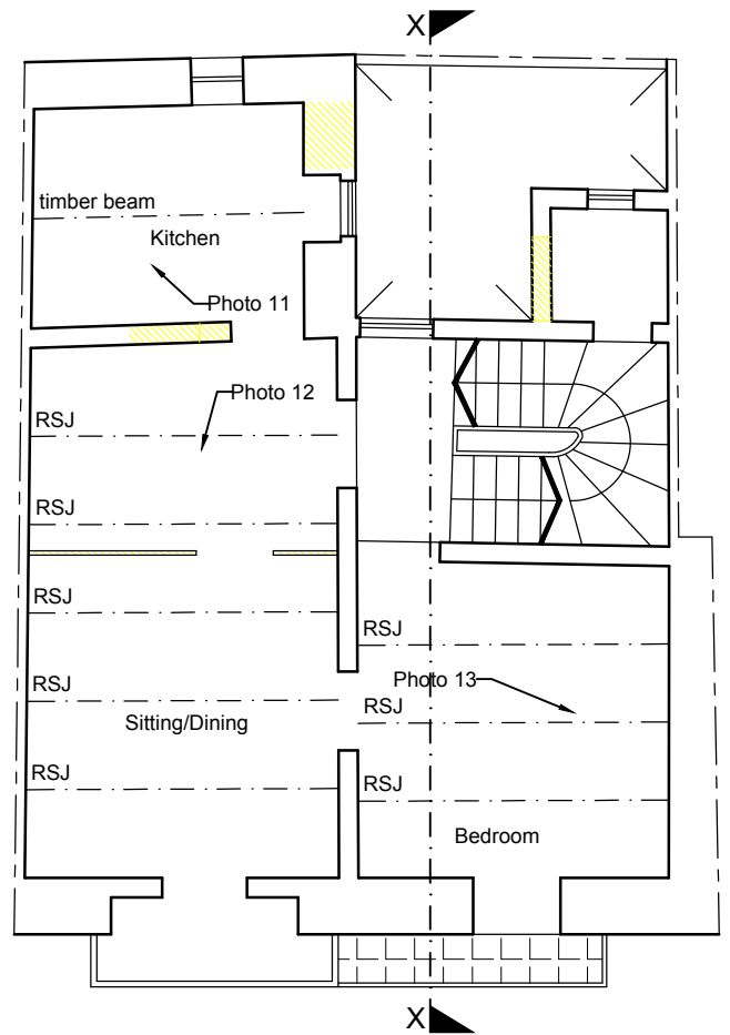
Existing Third Floor SCALE 1:100
