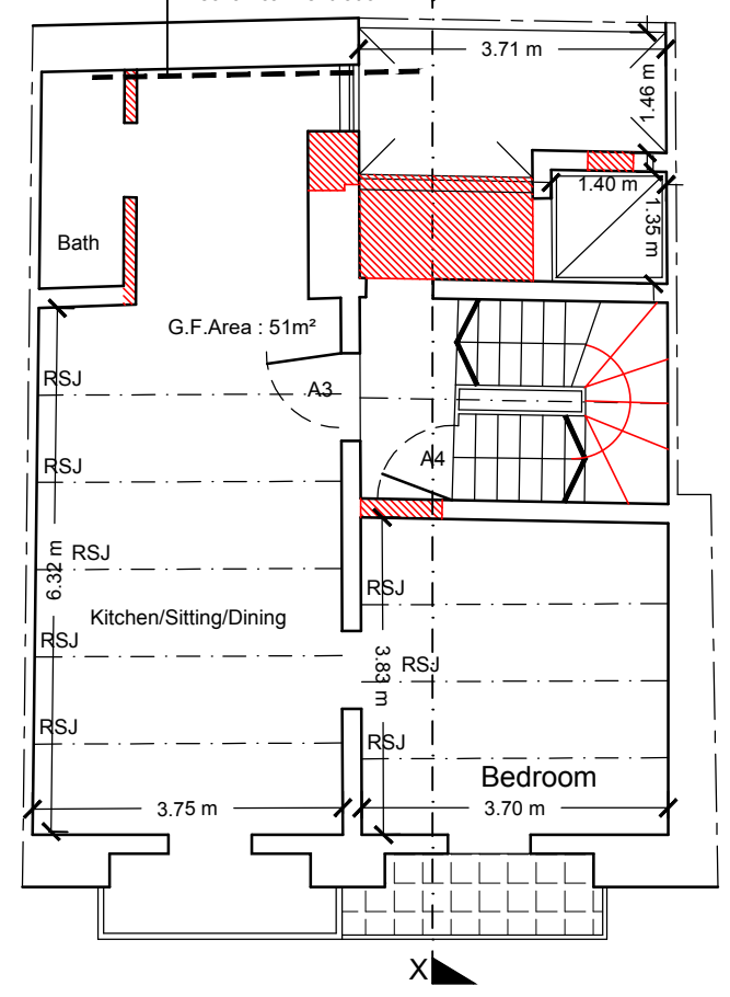
Proposed Fourth Floor SCALE 1:100
