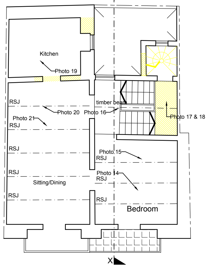
Existing Fourth Floor SCALE 1:100
