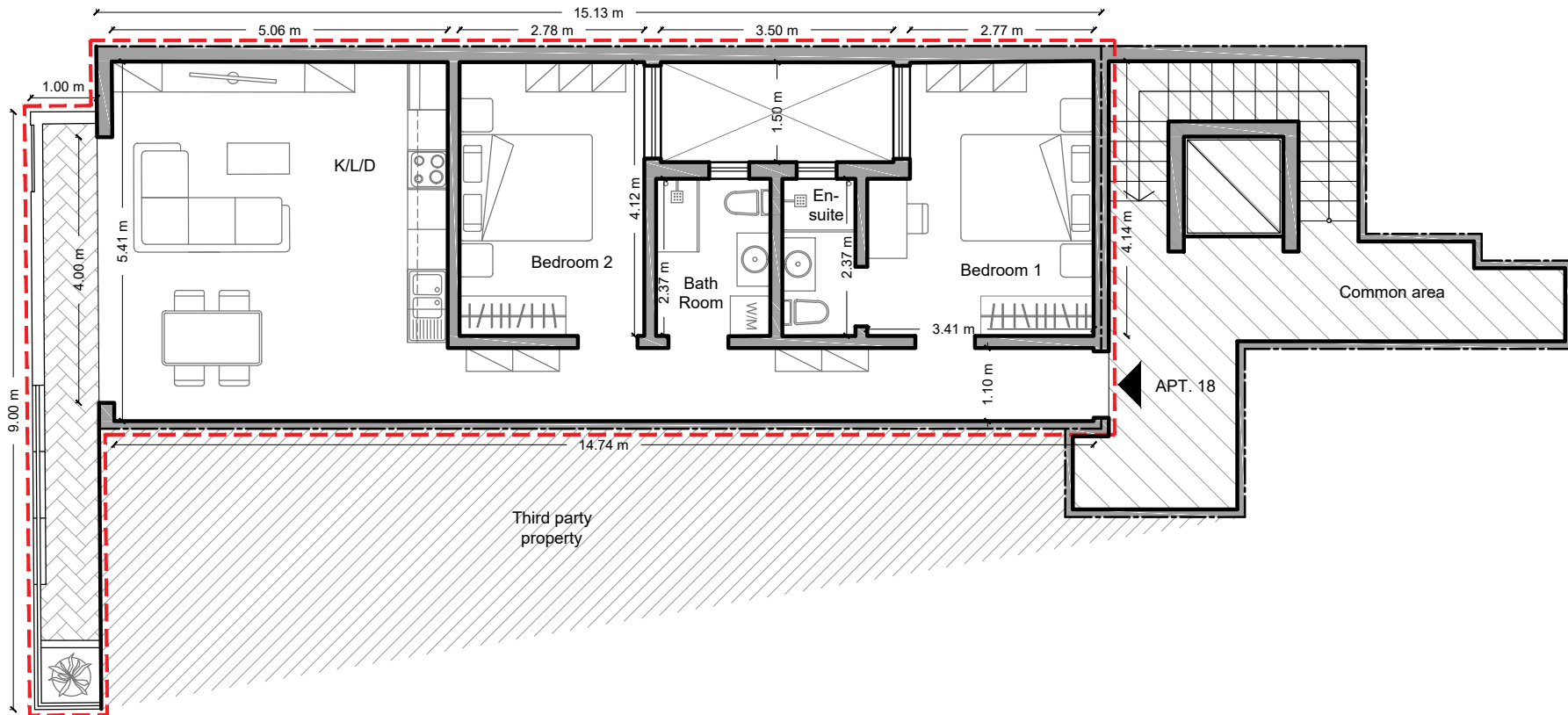
Approved Third Floor Level 1:100
