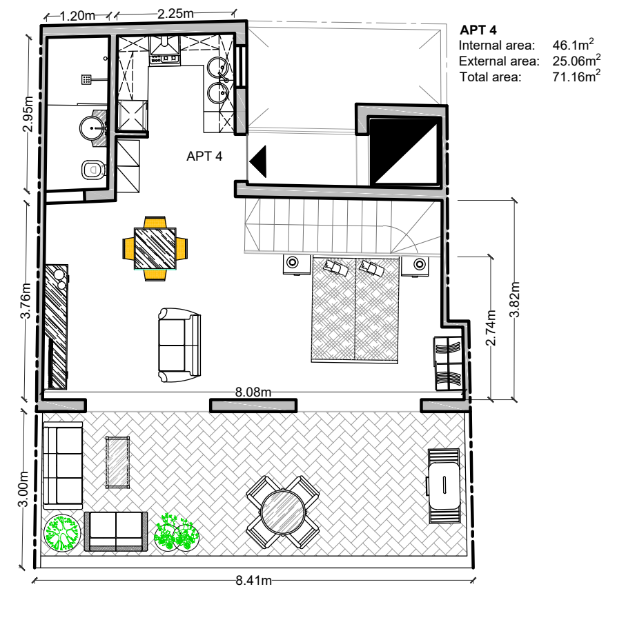
Fifth Floor 1:100
