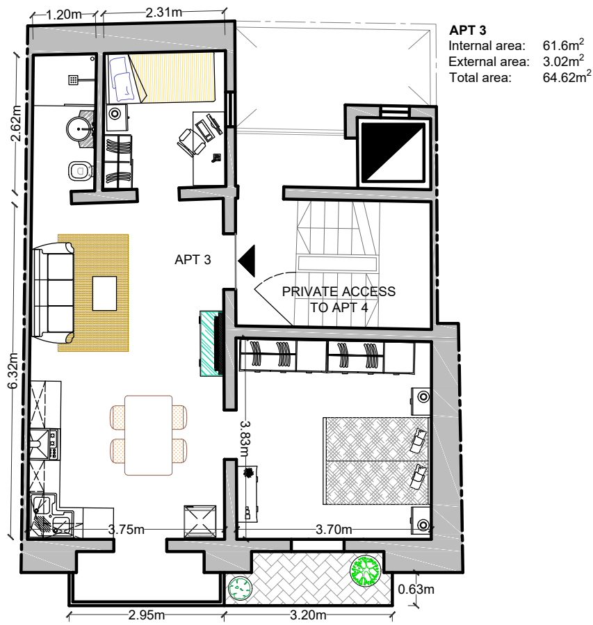
Fourth Floor 1:100
