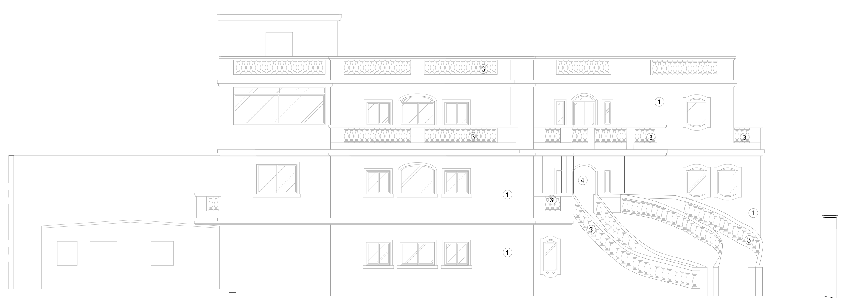
EXISTING ELEVATION C SCALE 1:100
