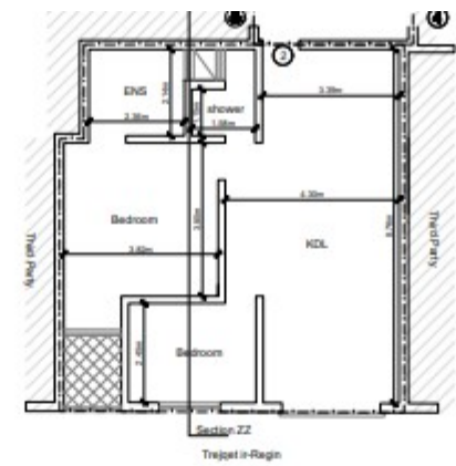
Proposed Upper Ground Floor Level Scale 1:100 Internal area - 76.21sm
