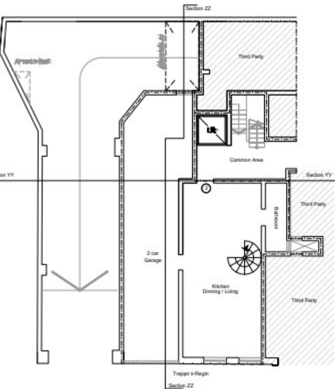
As Approved Lower Ground Floor Level - PA 7607 / 07 Scale 1:100
