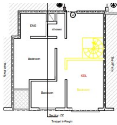
Proposed Upper Ground Floor Level - Conventional Colors Scale 1:100
