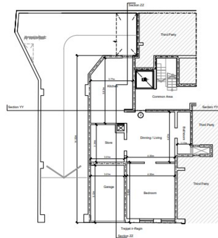
Proposed Lower Ground Floor Level Scale 1:100 APT Internal area - Rd. 48sm
