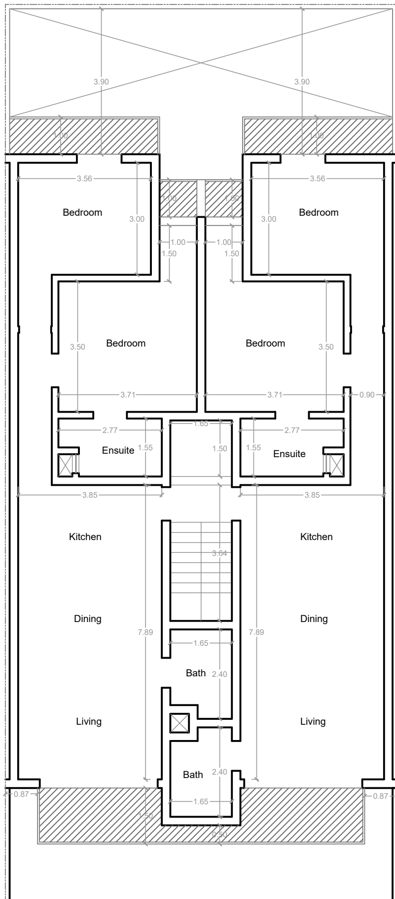
Proposed Third floor scale 1:100
