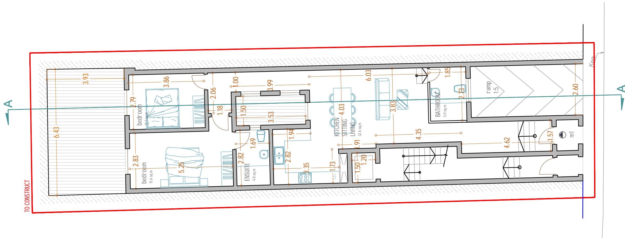
PROPOSED GROUND FLOOR UNIT SCALE 1:100
