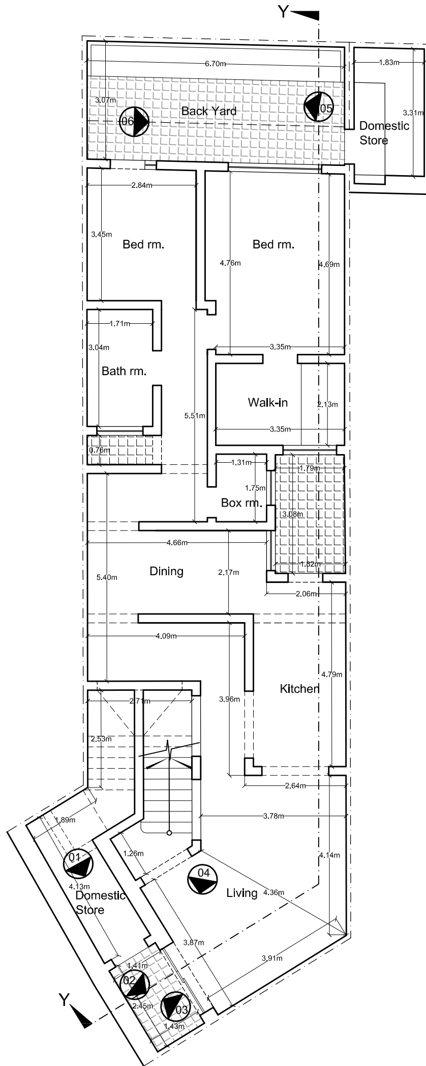
Existing Floor Plan at Basement Level Scale 1:100
