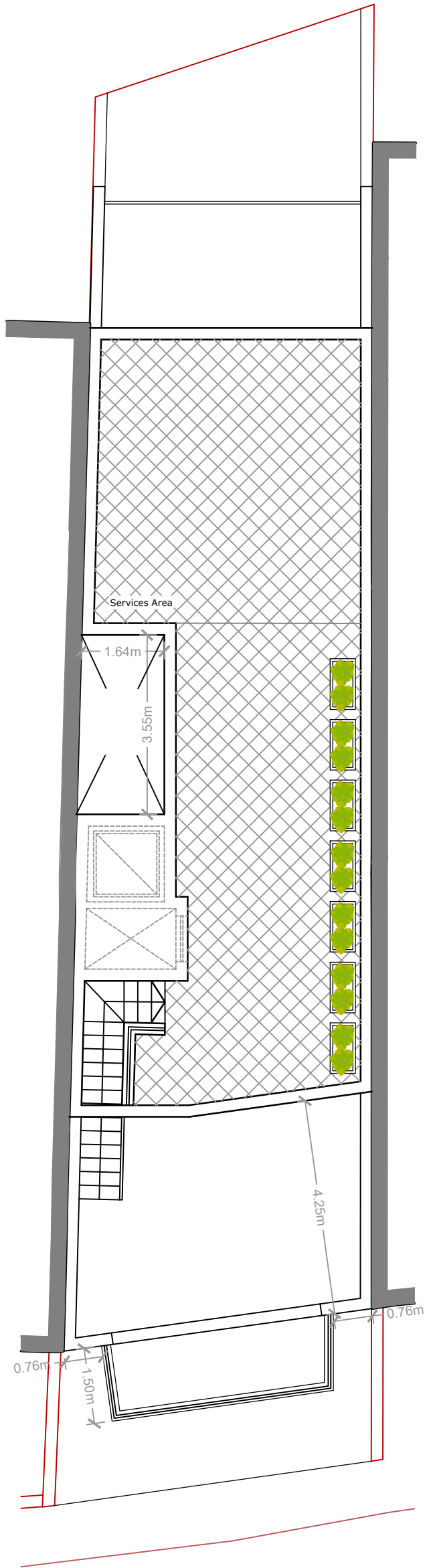
Proposed Roof Level Scale 1:100
