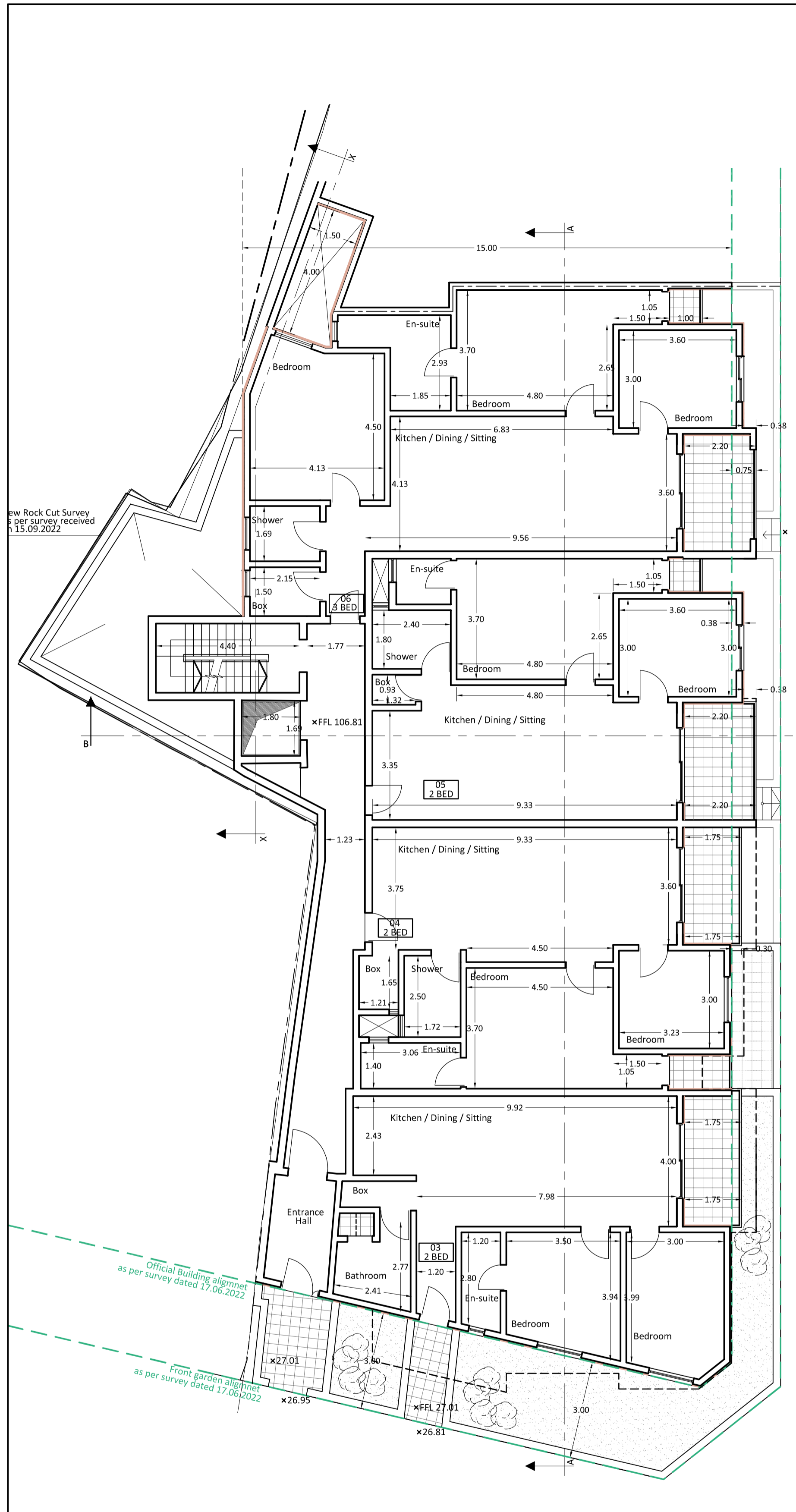
LEVEL 3 SCALE 1:100 PROPOSED
