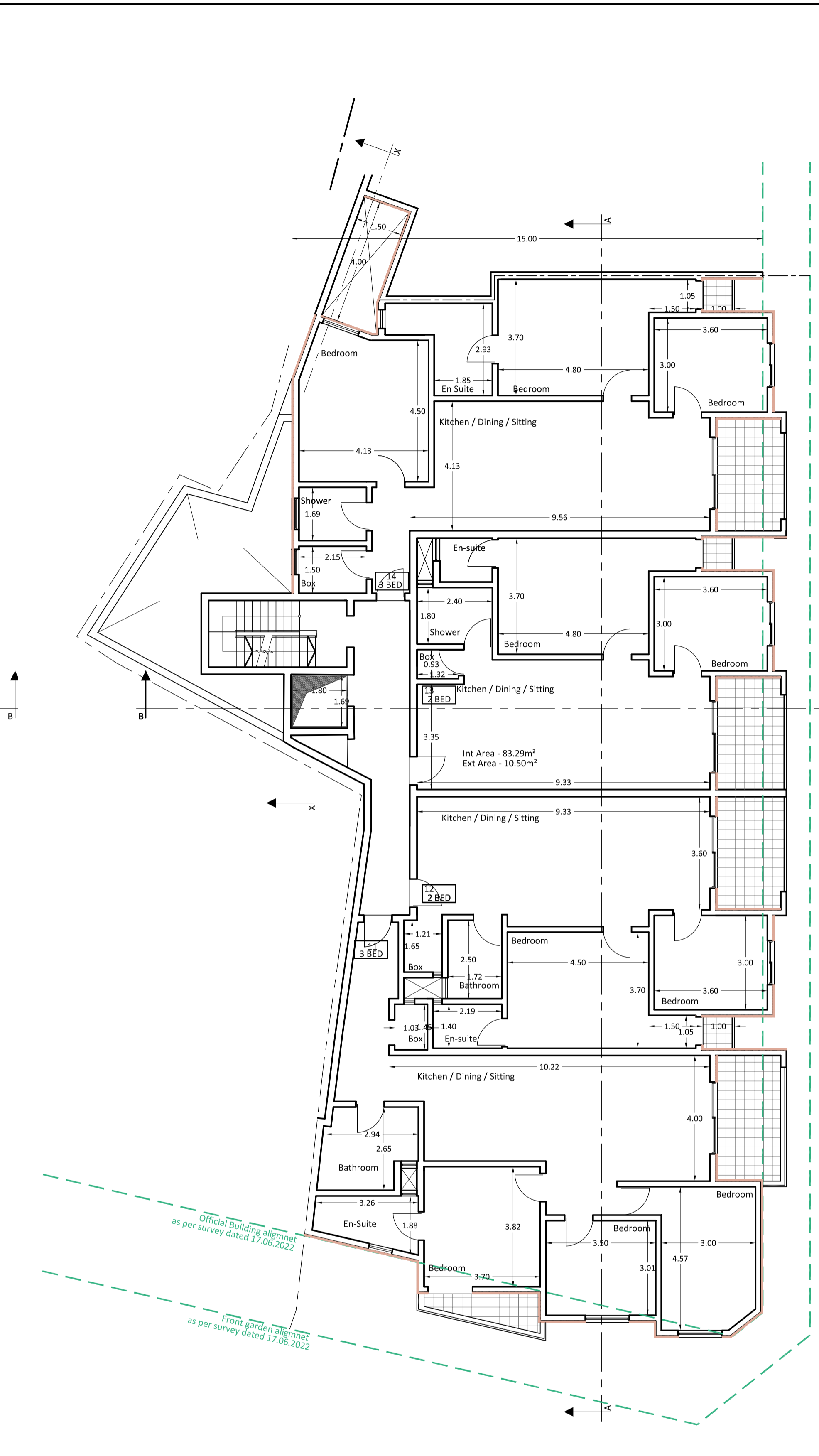
LEVEL 5 SCALE 1:100 PROPOSED
