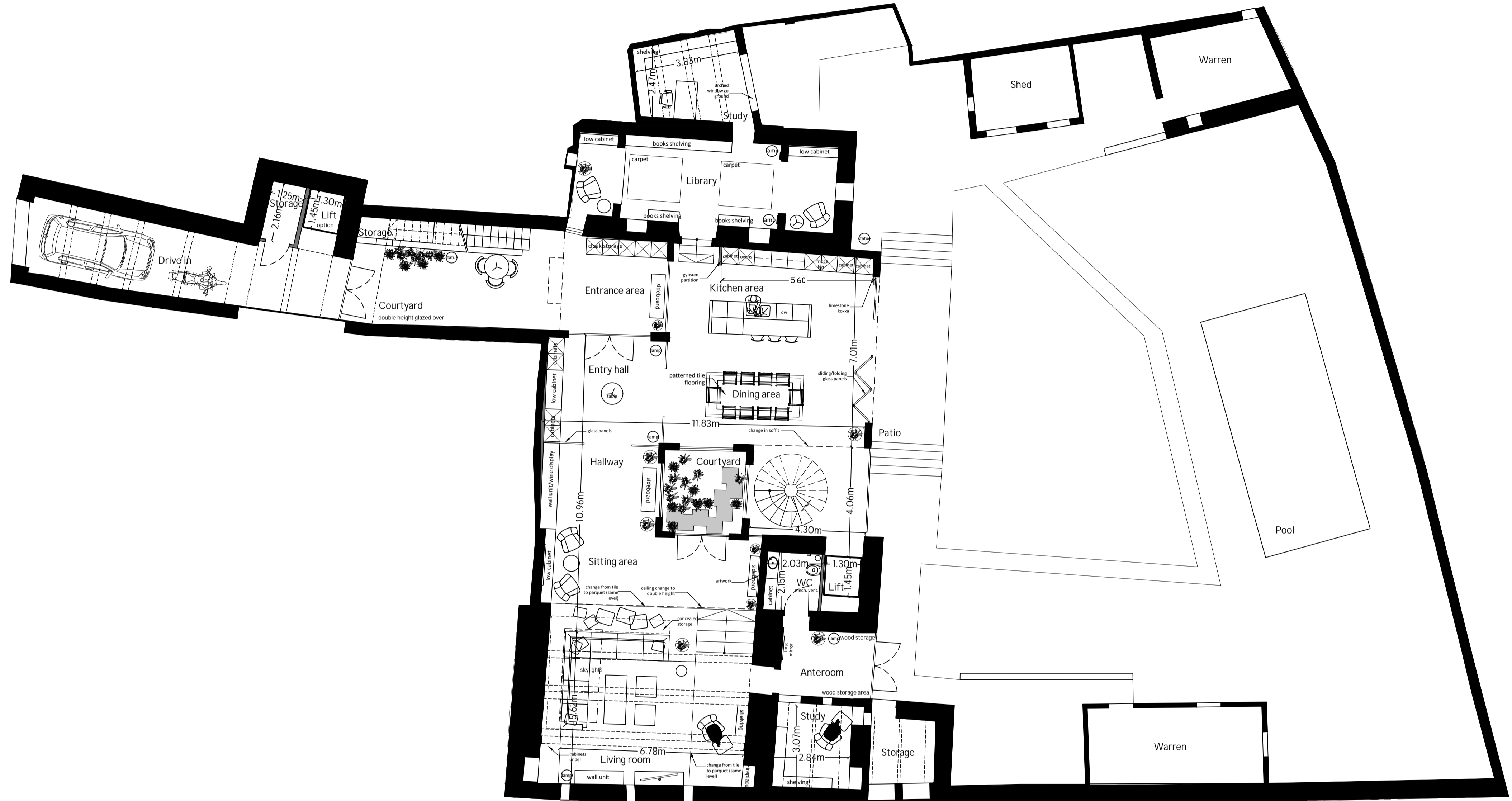
A1 | PROPOSED GROUND FLOOR LAYOUT 01 | SCALE 1:100
