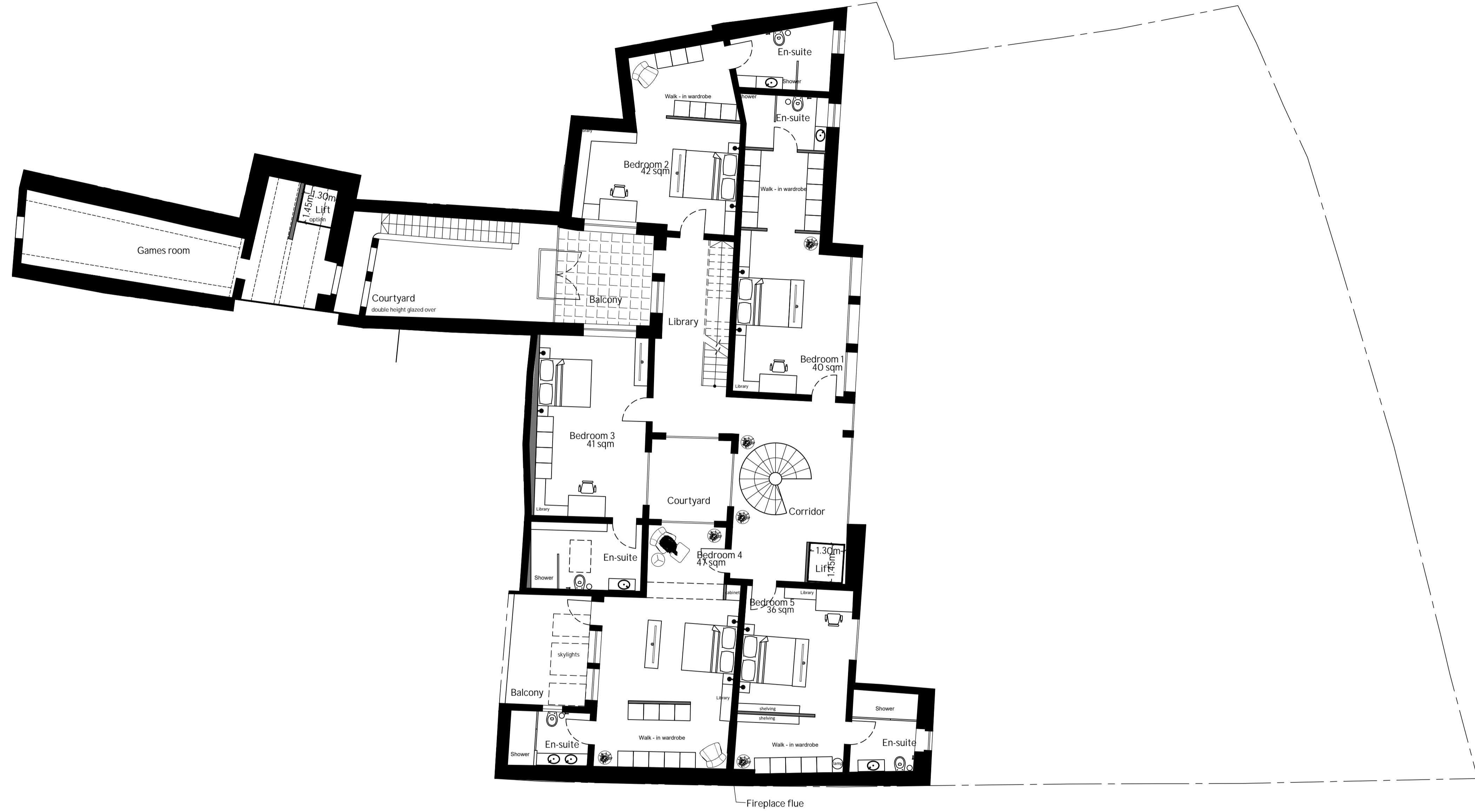
A2 | PROPOSED FIRST FLOOR LAYOUT 01 SCALE 1:100
