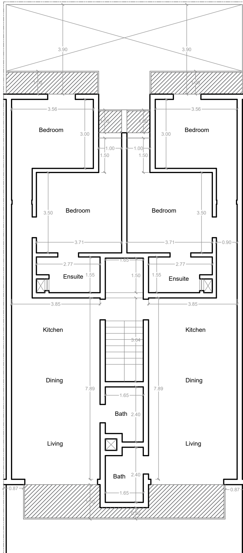
Proposed Second floor scale 1:100
